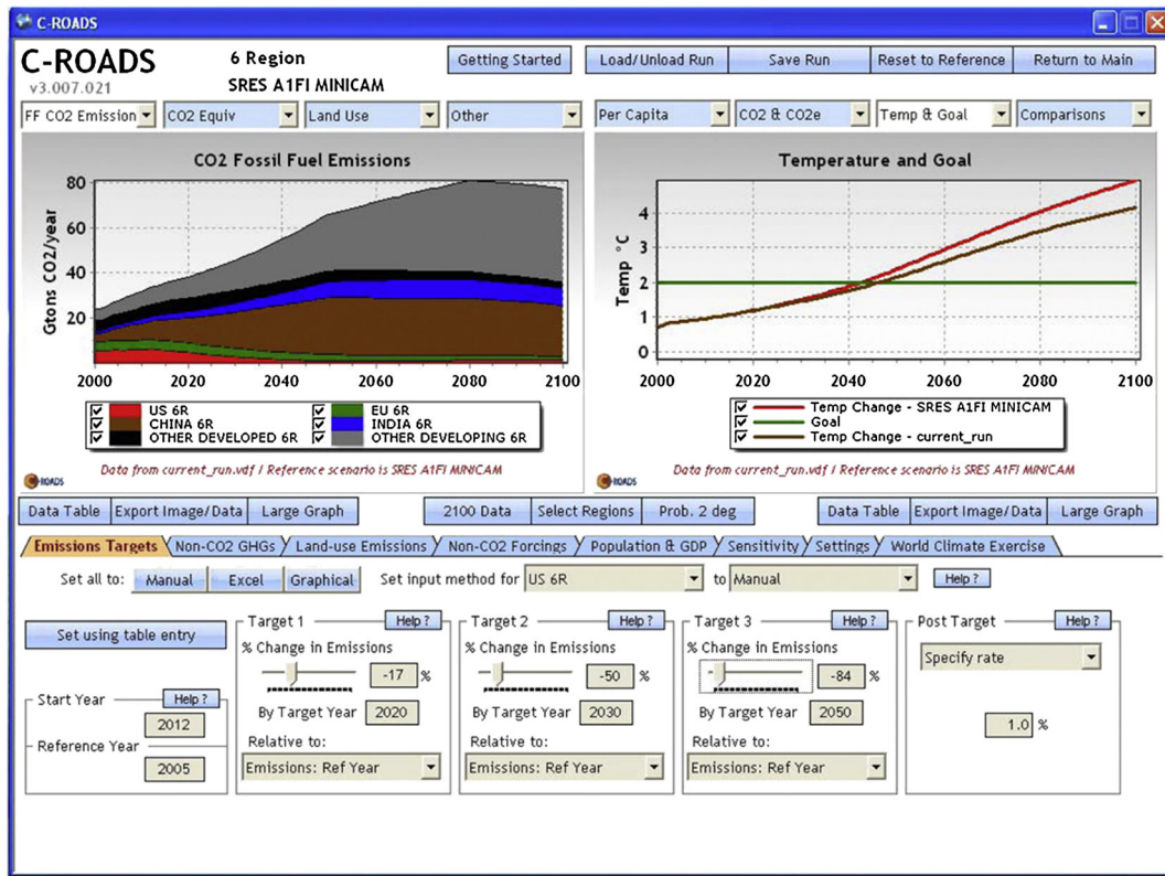
Fig. 5. C-ROADS interface
